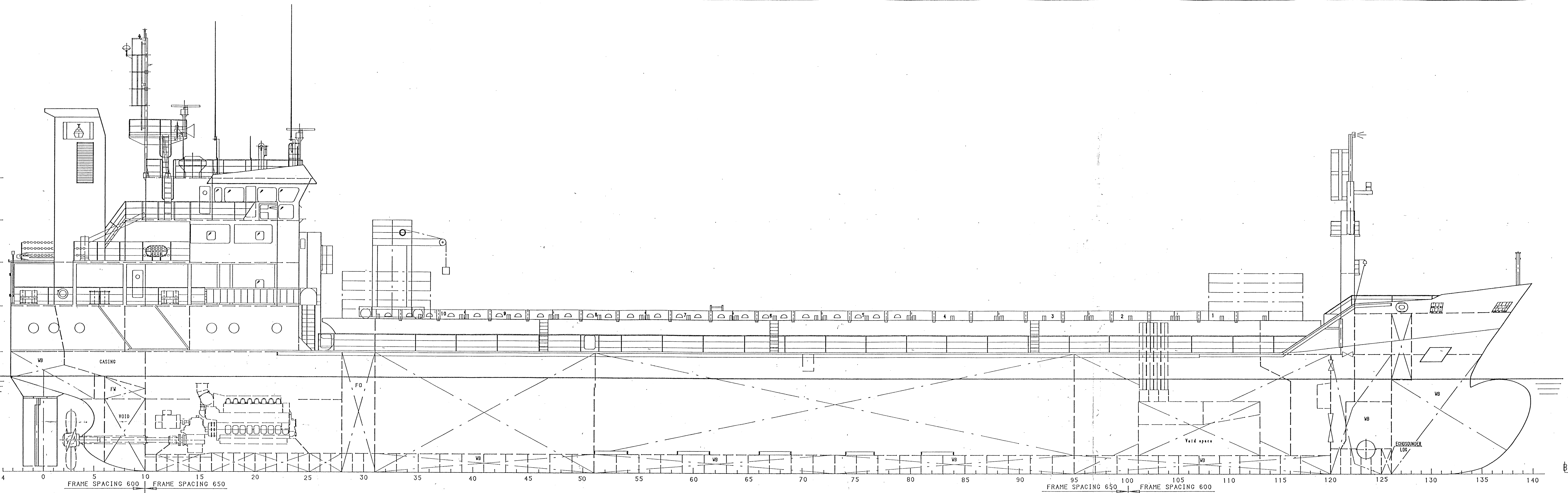
MAIN DECK
