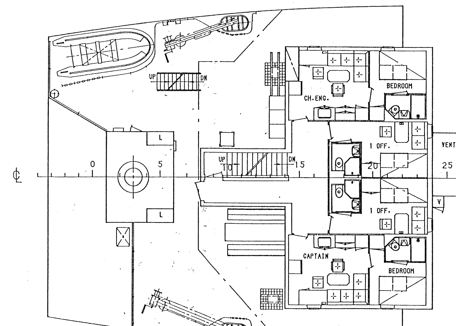
2 nd POOP DECK
