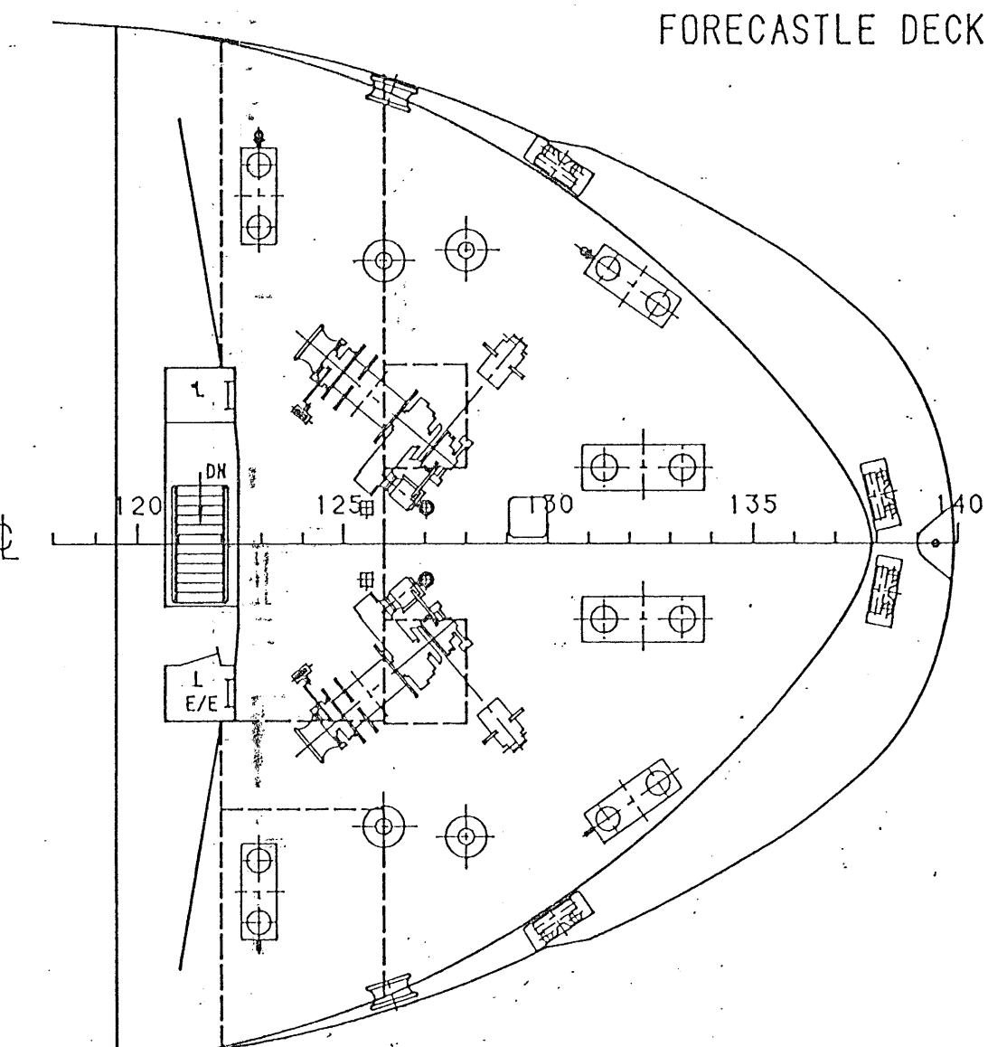
FORECASTLE DECK
