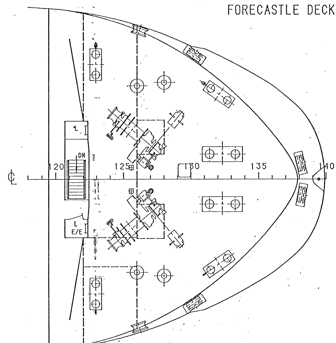
FORECASTLE DECK
