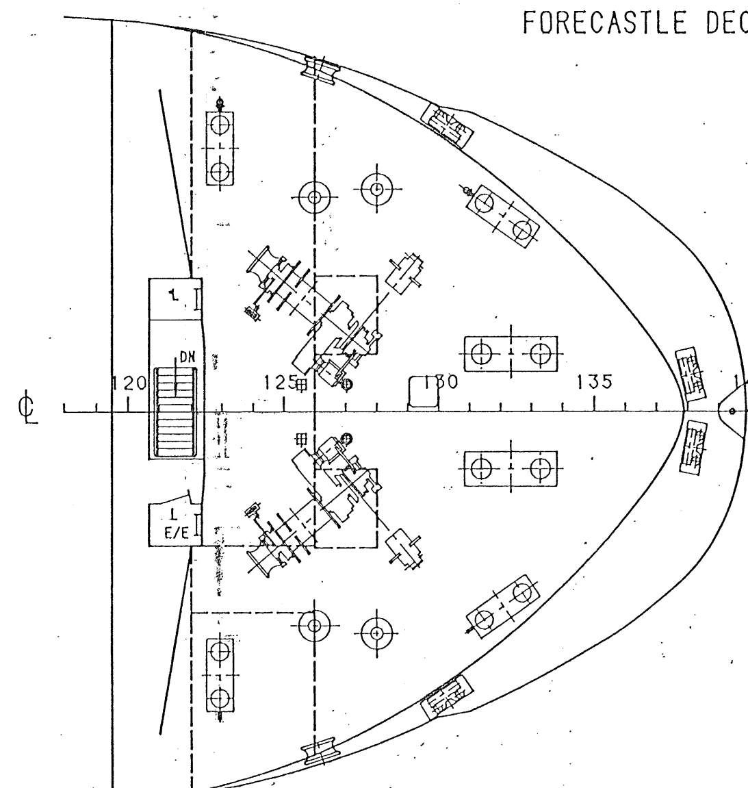
FORECASTLE DECK
