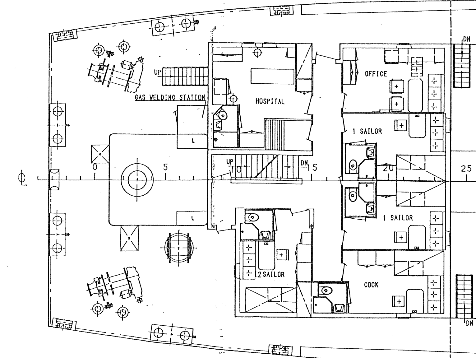
1 st POOP DECK
