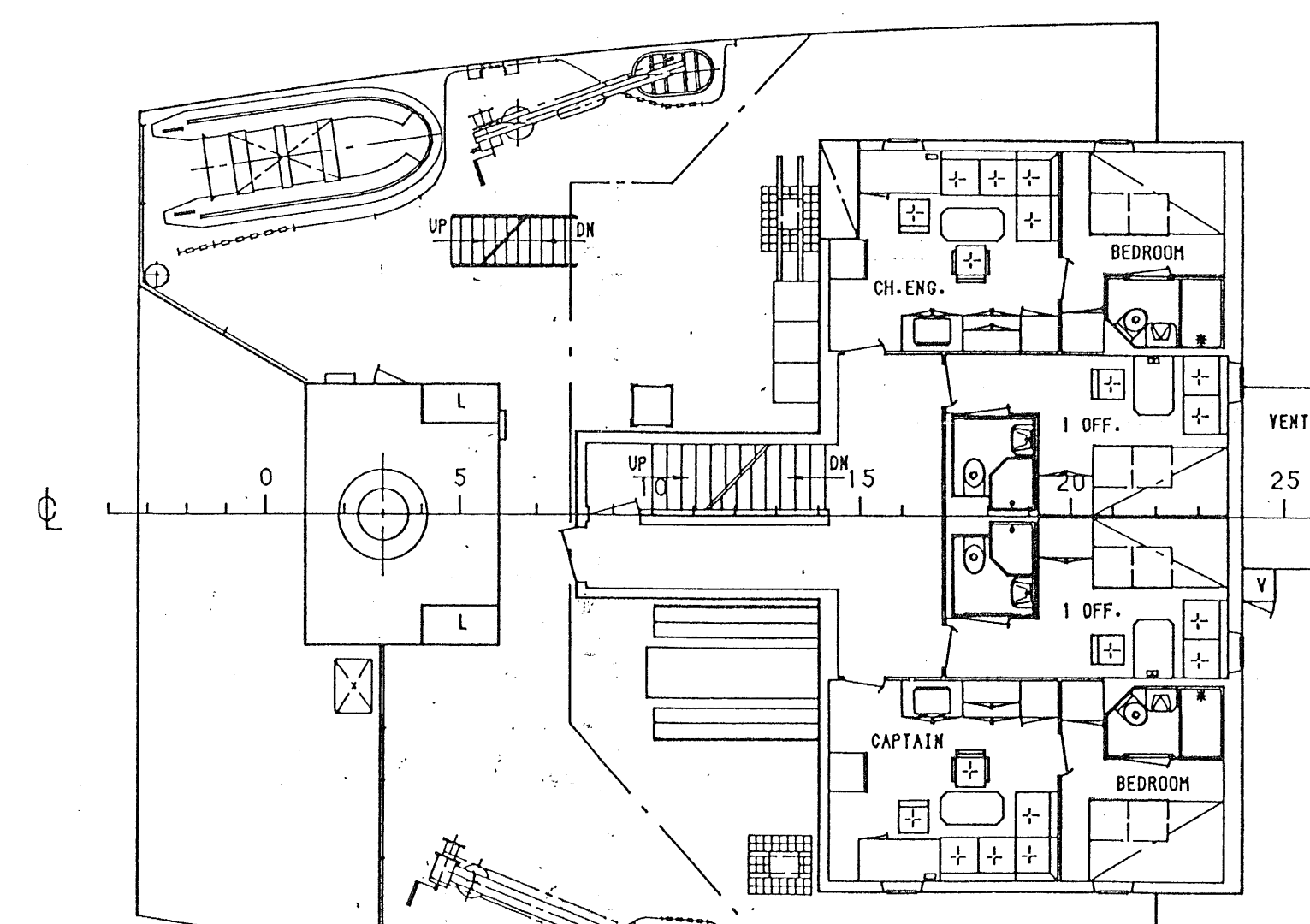
2 nd POOP DECK
