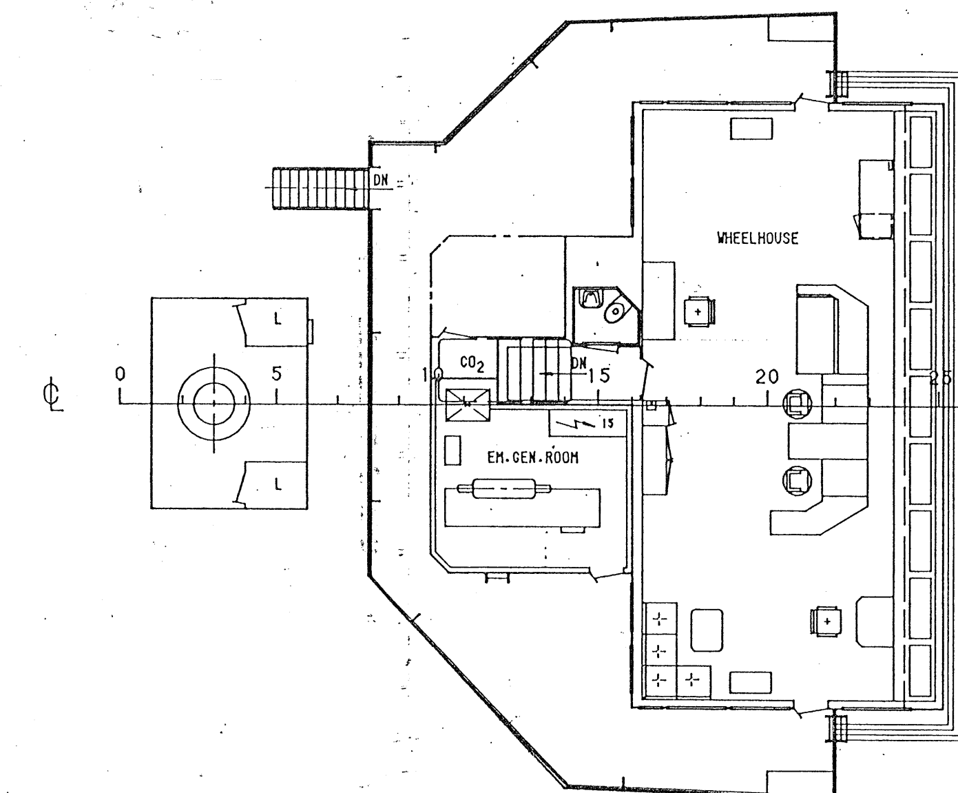
2 nd POOP DECK
