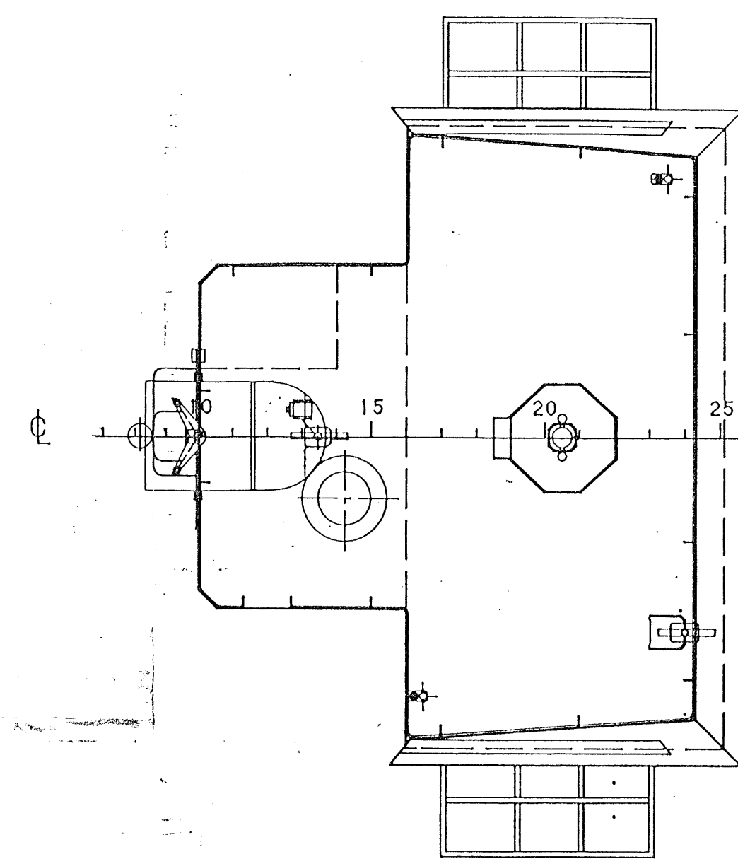
BRIDGE DECK
