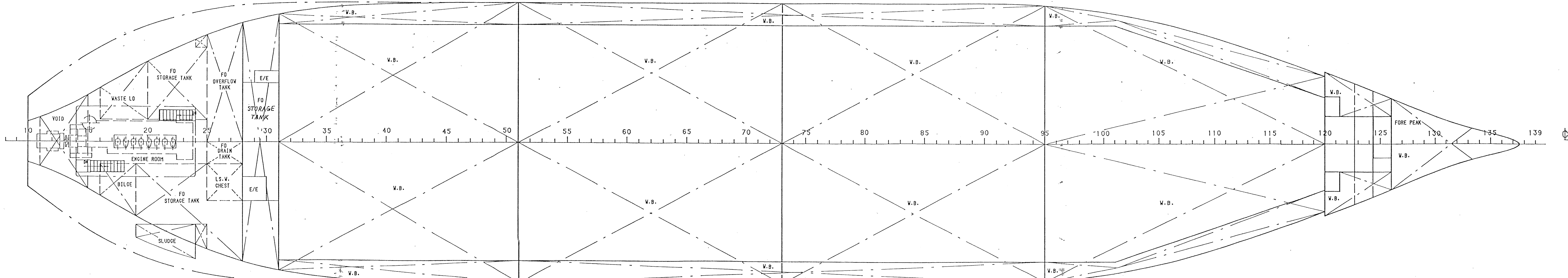
TANKS
