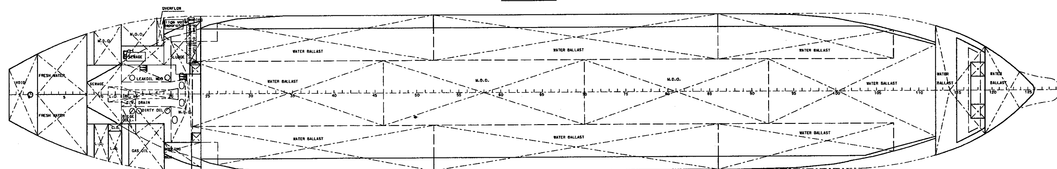
TANKTOP
