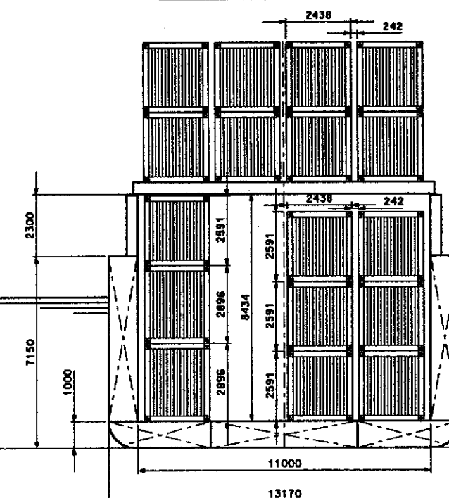
CROSS SECTION
